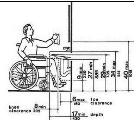
Fig. 31 Lavatory Clearances
